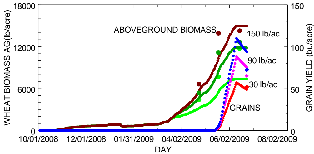
Figure 7. Time series of aboveground biomass simulated and hand measured for the fertilizer application scenarios 30, 90, and 150 lb/ac nitrogen. Simulated grain yields are shown and compared to machine harvested yield.
