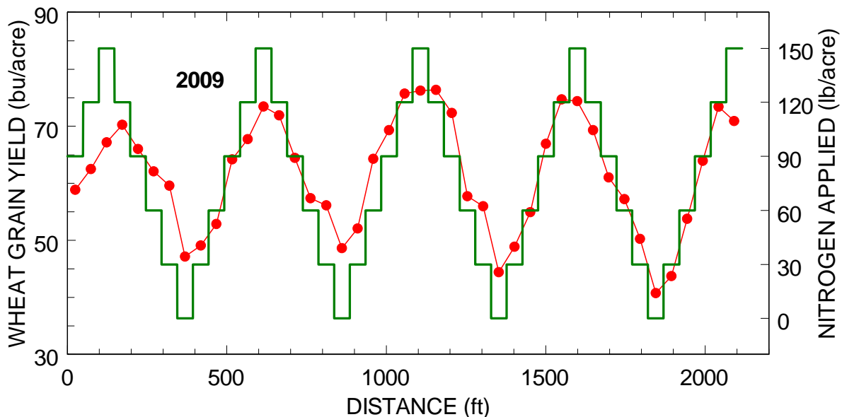
Figure 1. Spatial design of the fertilizer application rate and wheat grain yield measured in summer 2009.
