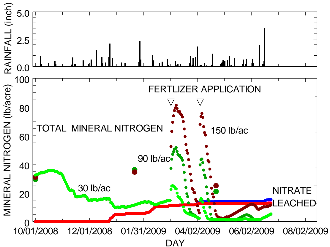
Figure 8. Mineral soil nitrogen in the entire profile and cumulative nitrate leaching during the growing season for the fertilizer scenarios 30, 90, and 150 lb/ac nitrogen.
