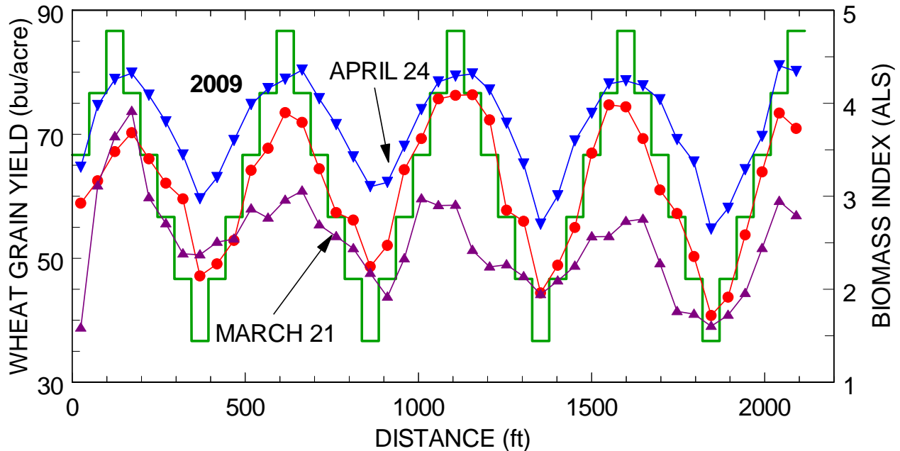
Figure 4. Wheat grain yield, nitrogen application rate and spatial pattern of biomass measured with the ALS at two different times.
