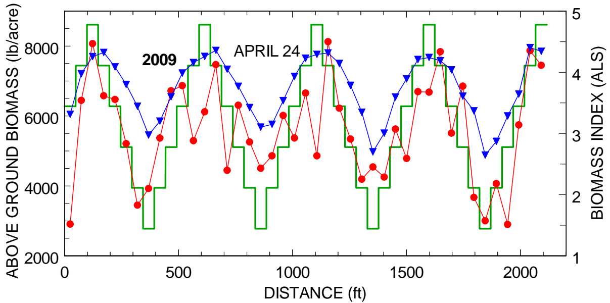
Figure 5. Biomass index measurements obtained with the ALS in comparison to hand-harvested aboveground biomass.
